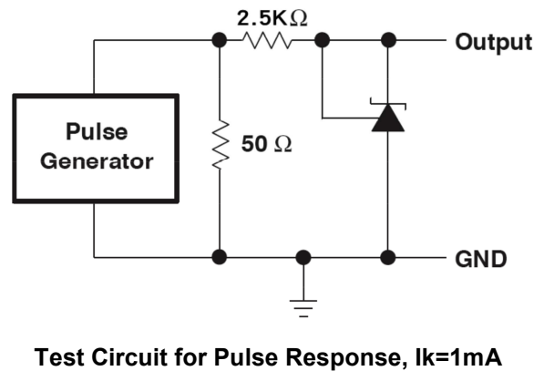
Figure 14. Pulse Response
