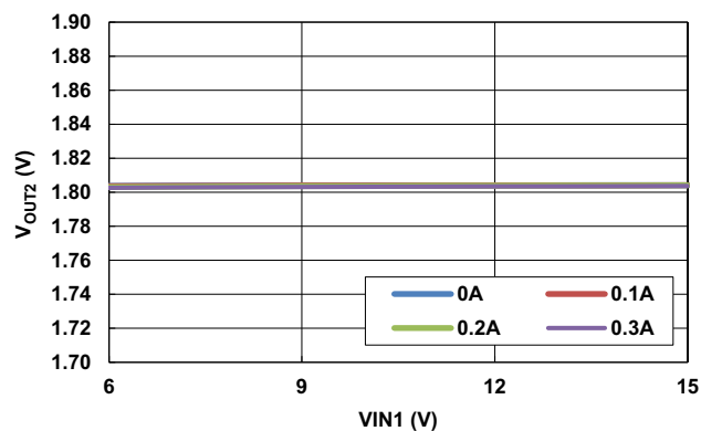
Figure 17. V_{OUT2} Two-Stage Line Regulation
