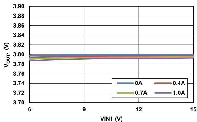
Figure 16. V_{OUT1} One-Stage Line Regulation
