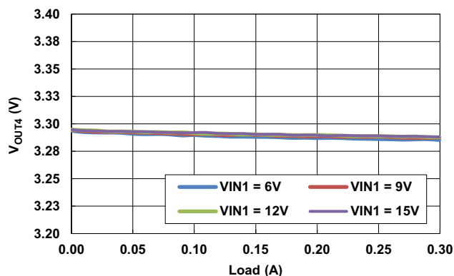
Figure 13. V OUT4 Load Regulation
