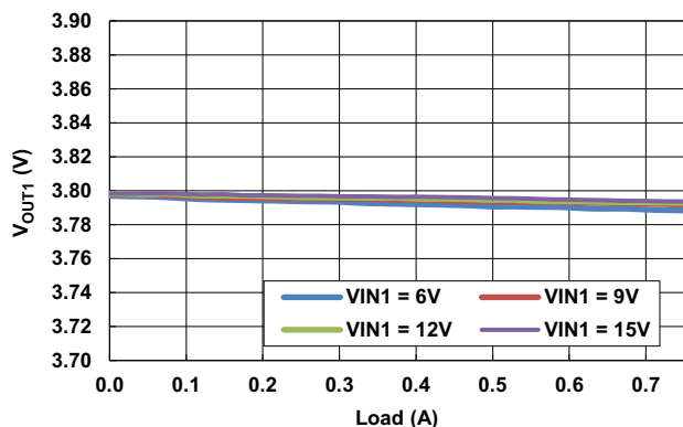
Figure 10. V OUT1 Load Regulation
