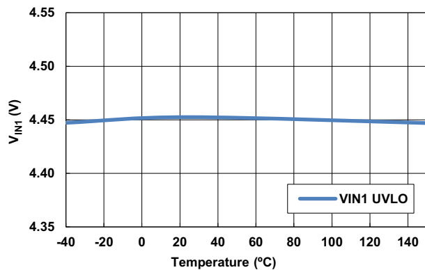
Figure 15. VIN1 UVLO Rising Edge vs Temperature
