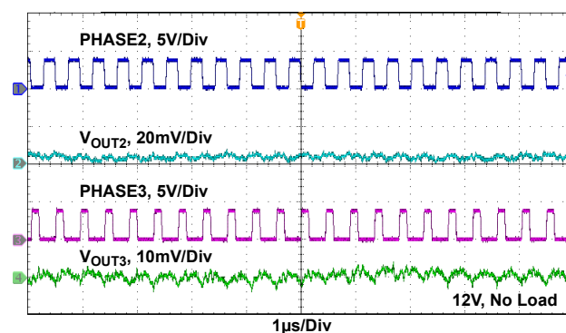
Figure 21. Switching: PHASE2, V_{OUT2} , PHASE3, V_{OUT3}
