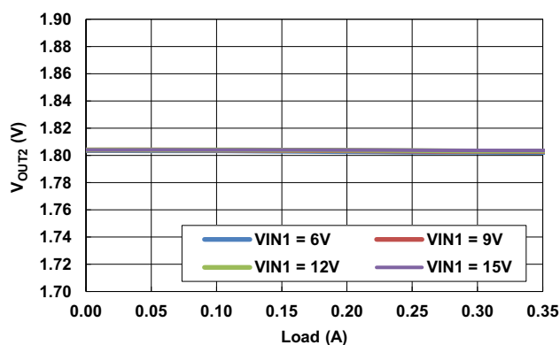
Figure 11. V OUT2 Load Regulation
