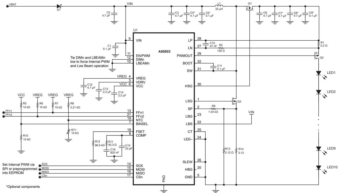
Single LED String Boost Controller with Configurable Internal PWM Dimming
