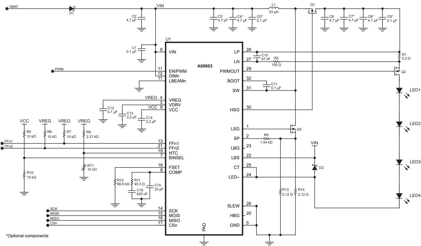
Single LED String Buck-Boost LED Controller with External PWM
