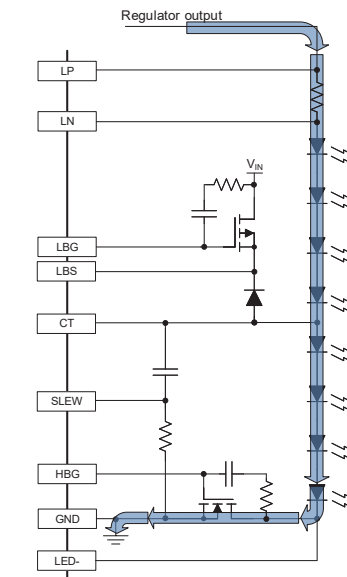
Figure 19: High-Beam LED Current Flow (Boost)
