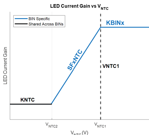
Figure 11: NTC Derating Programming Definitions
