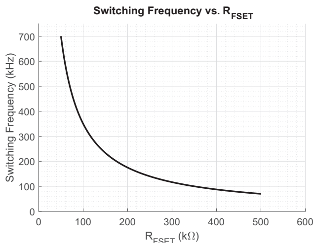
Figure 3: Switching Frequency vs. FSET Resistor
