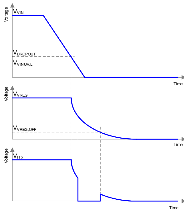
Figure 25: FFn1 and FFn2 behavior during shutdown when pulled up to VREG
