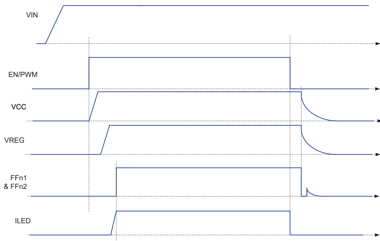
Figure 31: Startup and Shutdown with VREG_EN = 0
