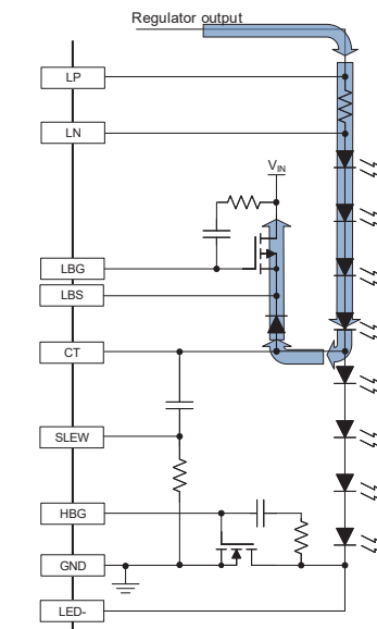
Figure 18: Low-Beam LED Current Flow (Buck-Boost)
