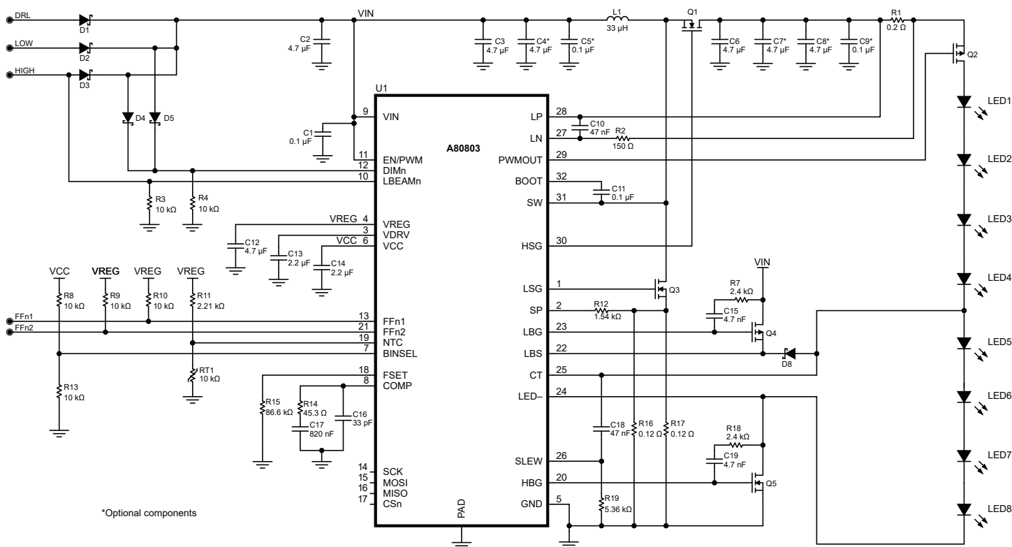
Figure 33: DRL, Low, High Tri-Level Lighting Application
