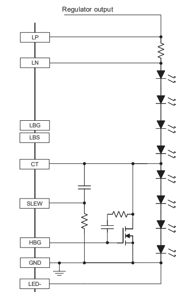
Figure 20: Low/High-Beam Control with Single MOSFET
