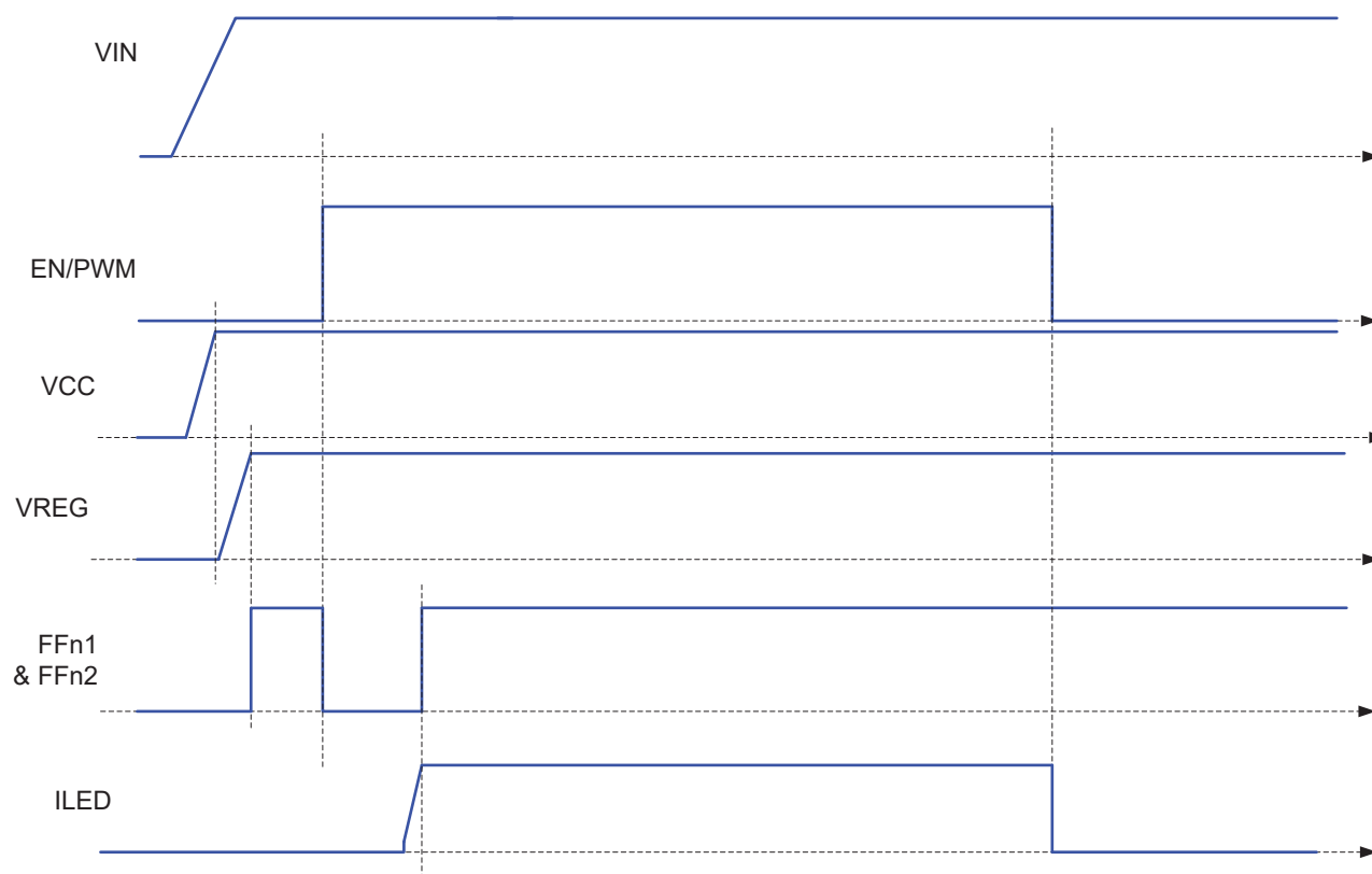
Figure 32: Startup and Shutdown with VREG_EN = 1
