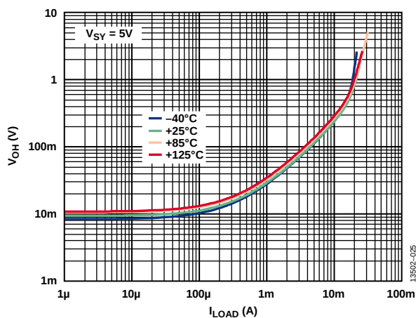
Figure 29. Output Voltage High ( V_{OH} ) to Supply Rail vs. Load Current ( I_{LOAD} ) over Temperature, V_{SY} = 5\text{ V}
