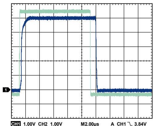
Figure 82. No Phase Reversal
