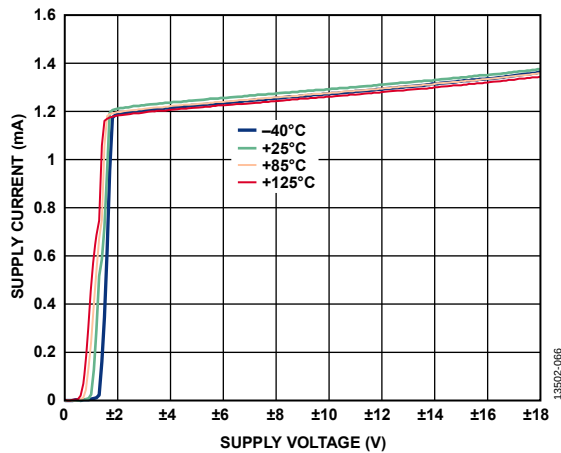
Figure 70. Supply Current ( I_{SV} ) vs. Supply Voltage ( V_{SY} ) for Various Temperatures (ADA4622-2)
