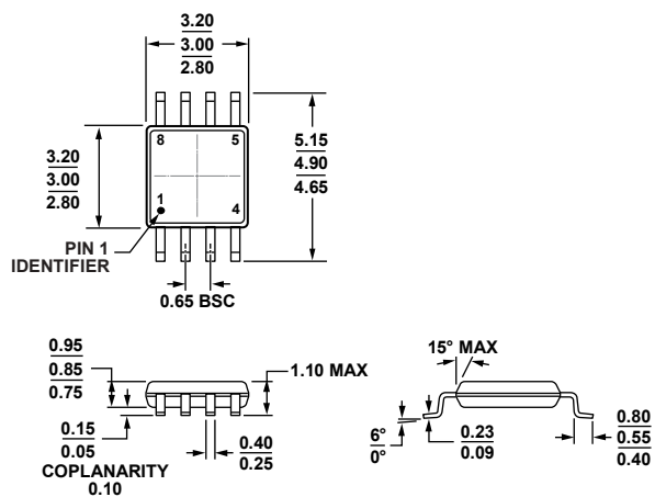
Figure 107. 8-Lead Mini Small Outline Package [MSOP] (RM-8)
