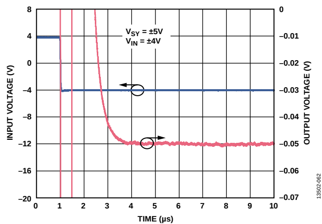
Figure 66. Negative Settling Time, A_V = -10 , V_{SY} = \pm 5V
