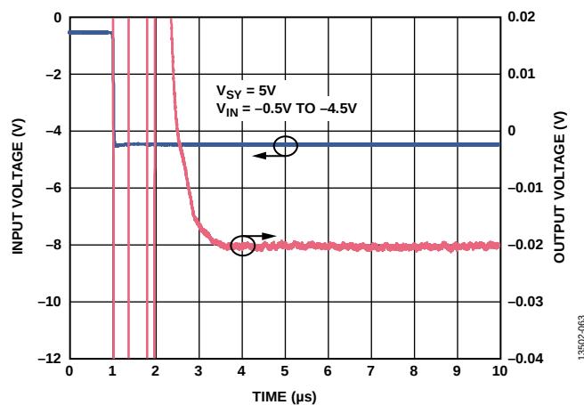
Figure 67. Negative Settling Time, A_V = -10 , V_{SY} = 5V
