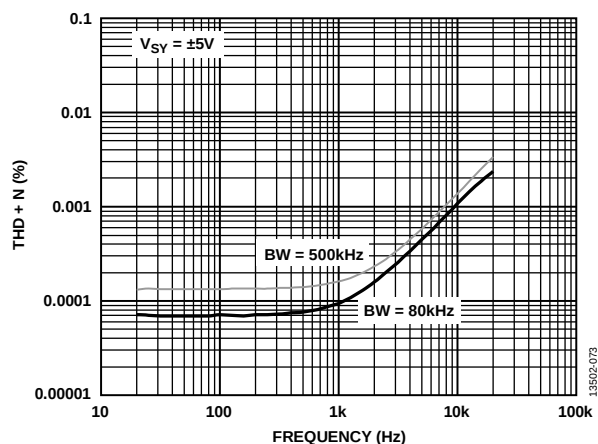
Figure 77. THD + N vs. Frequency, V_{SY} = \pm 5V
