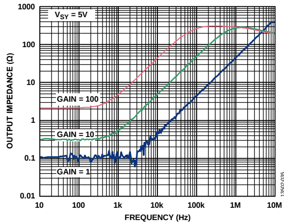
Figure 39. Output Impedance vs. Frequency, V_{SY} = 5\text{ V}
