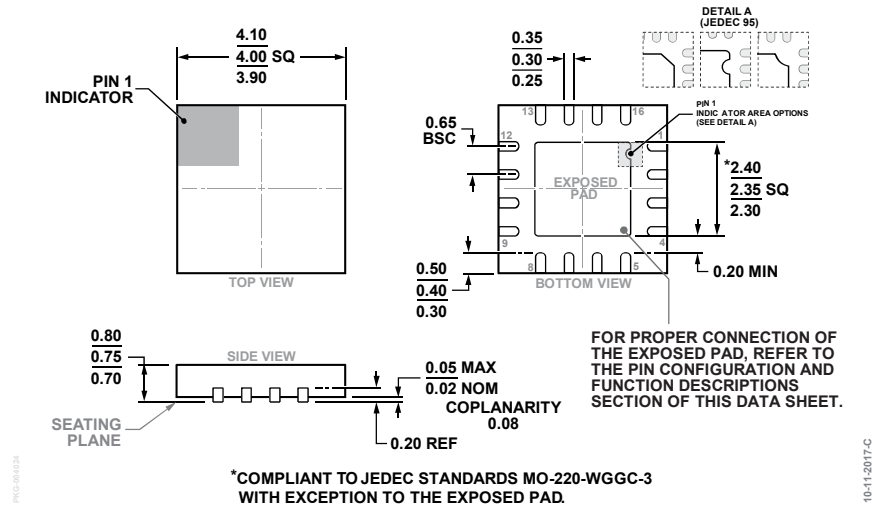
Figure 108. 16-Lead Lead Frame Chip Scale Package [LFCSP] 4 mm x 4 mm Body and 0.75 mm Package Height (CP-16-20)
