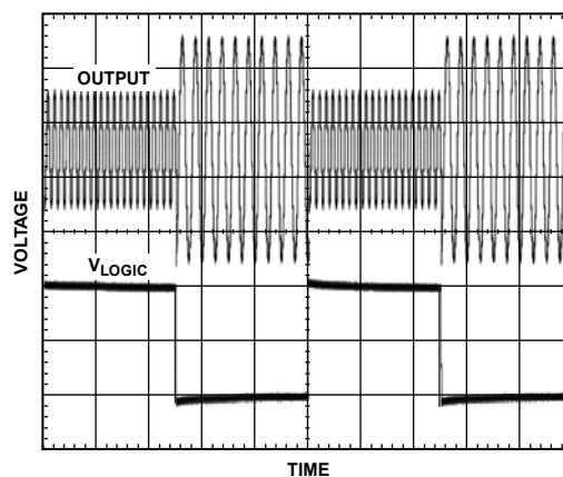
Figure 101. Multiplexed Output
