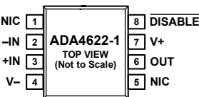
Figure 3. 8-Lead SOIC Pin Configuration, ADA4622-1
