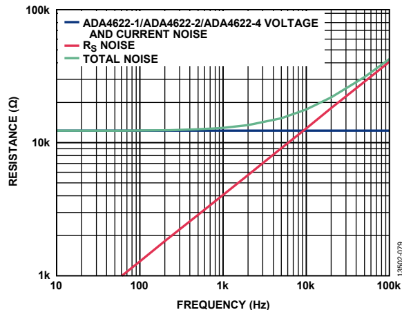
Figure 84. Total Noise vs. Source Resistance and Frequency
