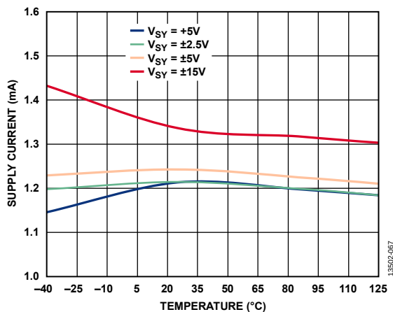
Figure 71. Supply Current ( I_{SV} ) vs. Temperature for Various Supply Voltages (ADA4622-2)
