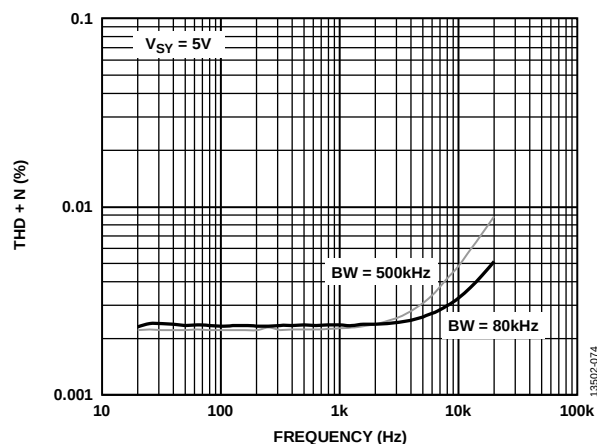
Figure 78. THD + N vs. Frequency, V_{SY} = 5V
