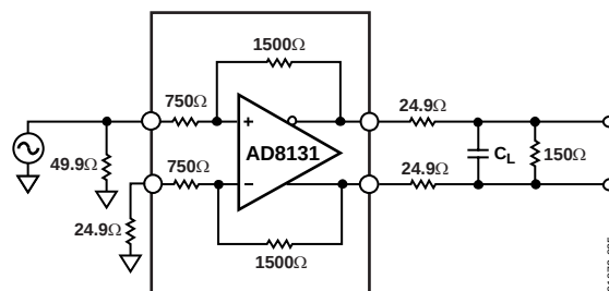
Figure 26. Capacitor Load Drive Test Circuit
