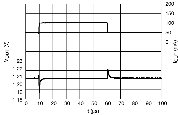
Figure 30. Load Transients, 1.2 V Version, I_{\text{OUT}} = 50 - 100 \text{ mA} , t_{\text{R}} = t_{\text{F}} = 0.5 \mu\text{s} , V_{\text{IN}} = 2.2 \text{ V}
