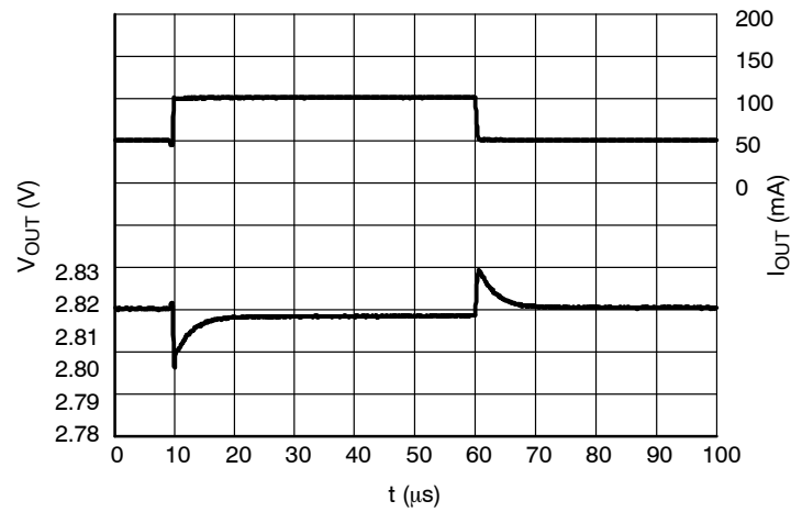
Figure 31. Load Transients, 2.8 V Version, I_{\text{OUT}} = 50 - 100 \text{ mA} , t_{\text{R}} = t_{\text{F}} = 0.5 \mu\text{s} , V_{\text{IN}} = 3.8 \text{ V}
