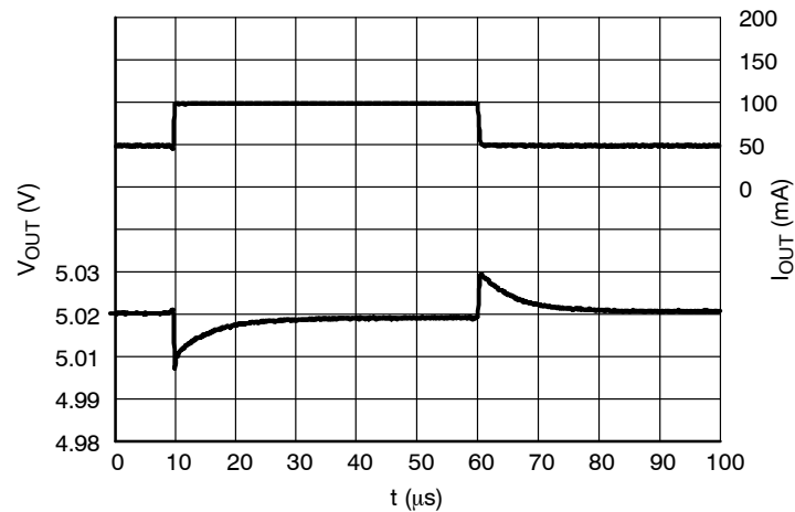
Figure 32. Load Transients, 5.0 V Version, I_{\text{OUT}} = 50 - 100 \text{ mA} , t_{\text{R}} = t_{\text{F}} = 0.5 \mu\text{s} , V_{\text{IN}} = 6.0 \text{ V}
