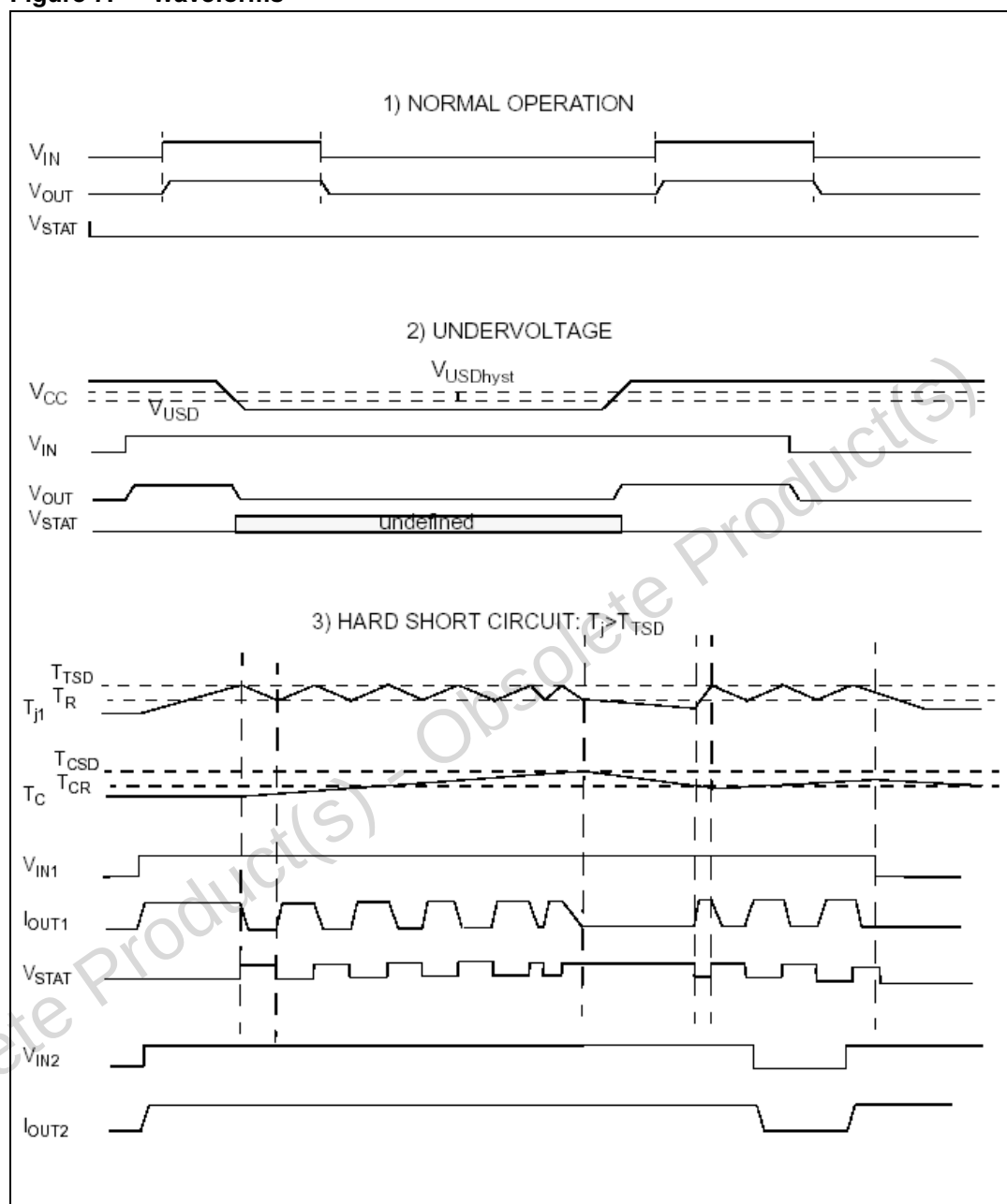
Figure 7. Waveforms
