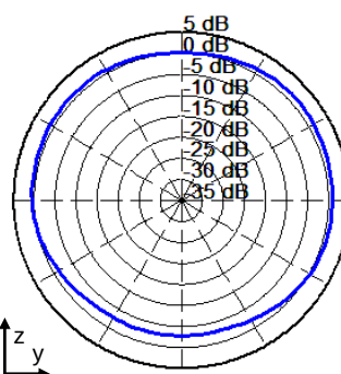
Phi = 90° Plane
