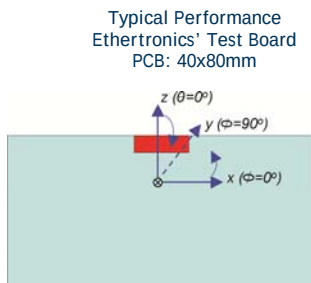
Phi = 0° Plane
