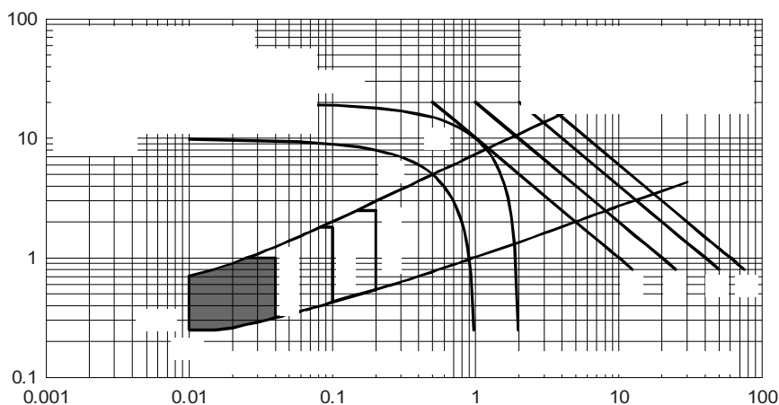
Fig. 11 - Gate Characteristics
