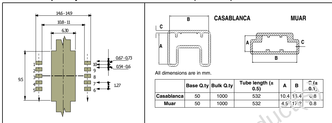
Figure 32. PowerSO-10 suggested pad layout
