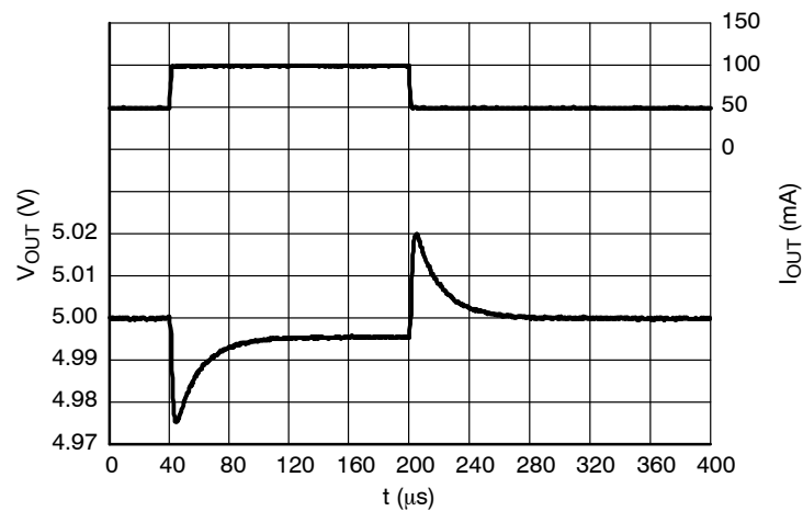
Figure 68. Load Transients, 5.0 V Version, I_{OUT} = 50 - 100 \text{ mA} , t_R = t_F = 0.5 \text{ } \mu\text{s} , V_{IN} = 8.0 \text{ V} , ECO = H
