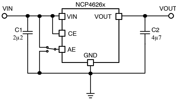
Figure 84. Typical Application Schematic
