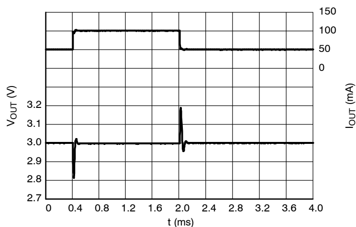
Figure 63. Load Transients, 3.0 V Version, I_{OUT} = 50 - 100 \text{ mA} , t_R = t_F = 0.5 \text{ } \mu\text{s} , V_{IN} = 6.0 \text{ V} , ECO = L
