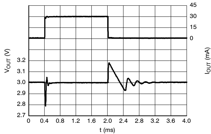
Figure 57. Load Transients, 3.0 V Version, I_{OUT} = 1 - 30 \text{ mA} , t_R = t_F = 0.5 \mu\text{s} , V_{IN} = 6.0 \text{ V} , ECO = L
