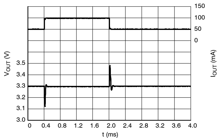
Figure 65. Load Transients, 3.3 V Version, I_{OUT} = 50 - 100 \text{ mA} , t_R = t_F = 0.5 \text{ } \mu\text{s} , V_{IN} = 6.3 \text{ V} , ECO = L
