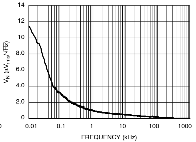
Figure 46. Output Voltage Noise, 3.0 V Version, V_{IN} = 6.0\text{ V} , I_{OUT} = 30\text{ mA} , ECO = H
