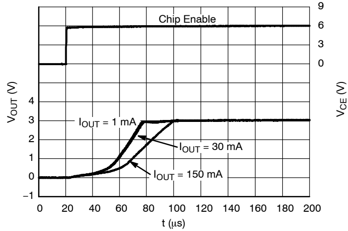
Figure 76. Start-up, 3.0 V Version, V_{IN} = 6.0\text{ V} , ECO = H
