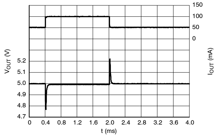
Figure 67. Load Transients, 5.0 V Version, I_{OUT} = 50 - 100 \text{ mA} , t_R = t_F = 0.5 \text{ } \mu\text{s} , V_{IN} = 8.0 \text{ V} , ECO = L
