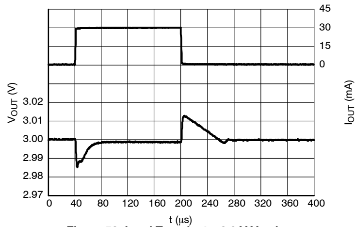
Figure 58. Load Transients, 3.0 V Version, I_{OUT} = 1 - 30 \text{ mA} , t_R = t_F = 0.5 \mu\text{s} , V_{IN} = 6.0 \text{ V} , ECO = H
