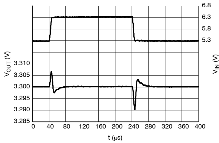
Figure 54. Line Transients, 3.3 V Version, t_R = t_F = 5 \mu s, I_{OUT} = 30 mA, ECO = H
