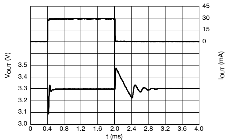
Figure 59. Load transients, 3.3 V version, I_{OUT} = 1 - 30 \text{ mA} , t_R = t_F = 0.5 \mu\text{s} , V_{IN} = 6.3 \text{ V} , ECO = L
