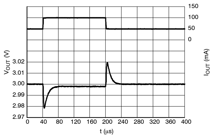
Figure 64. Load Transients, 3.0 V Version, I_{OUT} = 50 - 100 \text{ mA} , t_R = t_F = 0.5 \text{ } \mu\text{s} , V_{IN} = 6.0 \text{ V} , ECO = H
