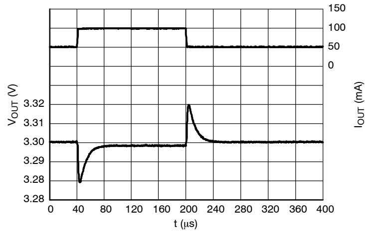
Figure 66. Load Transients, 3.3 V Version, I_{OUT} = 50 - 100 \text{ mA} , t_R = t_F = 0.5 \text{ } \mu\text{s} , V_{IN} = 6.3 \text{ V} , ECO = H
