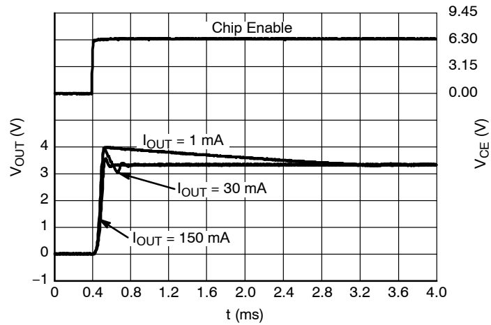
Figure 77. Start-up, 3.3 V Version, V_{IN} = 6.3\text{ V} , ECO = L
