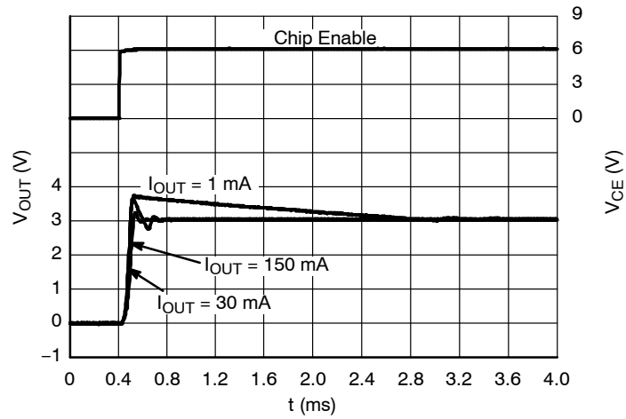
Figure 75. Start-up, 3.0 V Version, V_{IN} = 6.0\text{ V} , ECO = L
