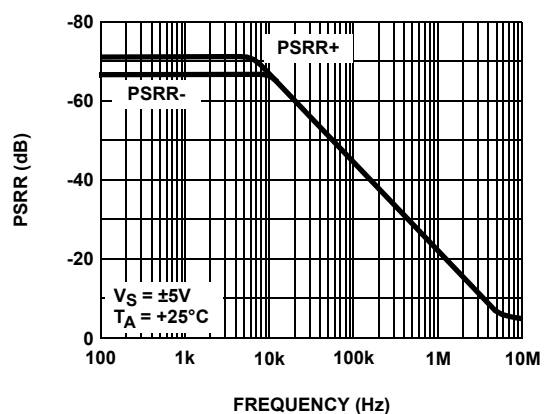
FIGURE 20. PSRR
