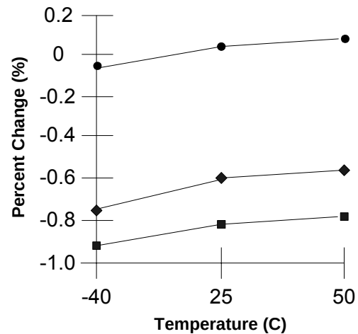
Chart 8: Oscillator Stability
