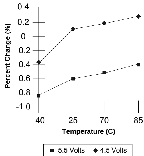
Chart 4: Oscillator Stability
