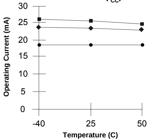
Chart 5: Record Mode Operating Current ( I_{CC} )
