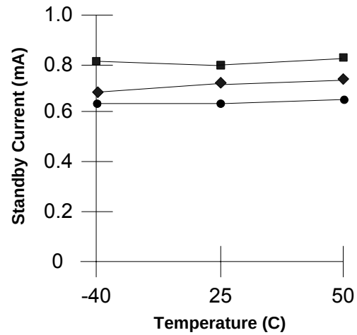
Chart 7: Standby Current ( I_{SB} )
