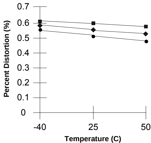
Chart 6: Total Harmonic Distortion
