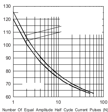
Fig. 5 - Maximum Non-Repetitive Surge Current
