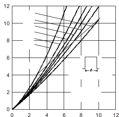
Fig. 4 - On-State Power Loss Characteristics
