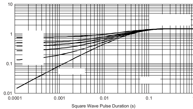
Fig. 8 - Thermal Impedance Z_{thJC} Characteristics
