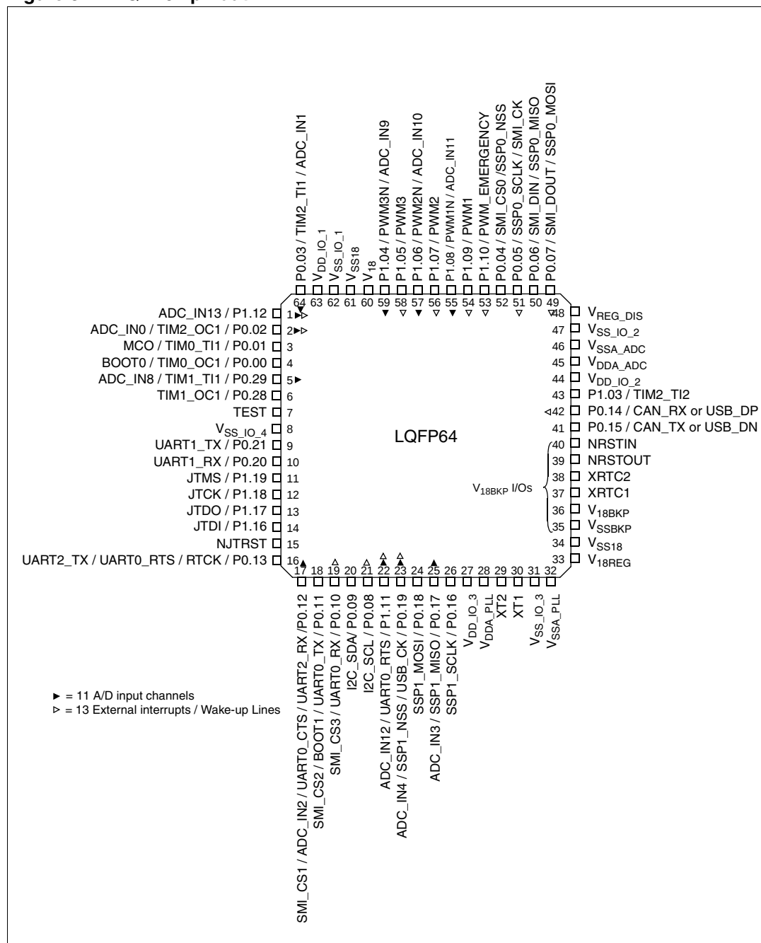
Figure 3. LQFP64 pinout
