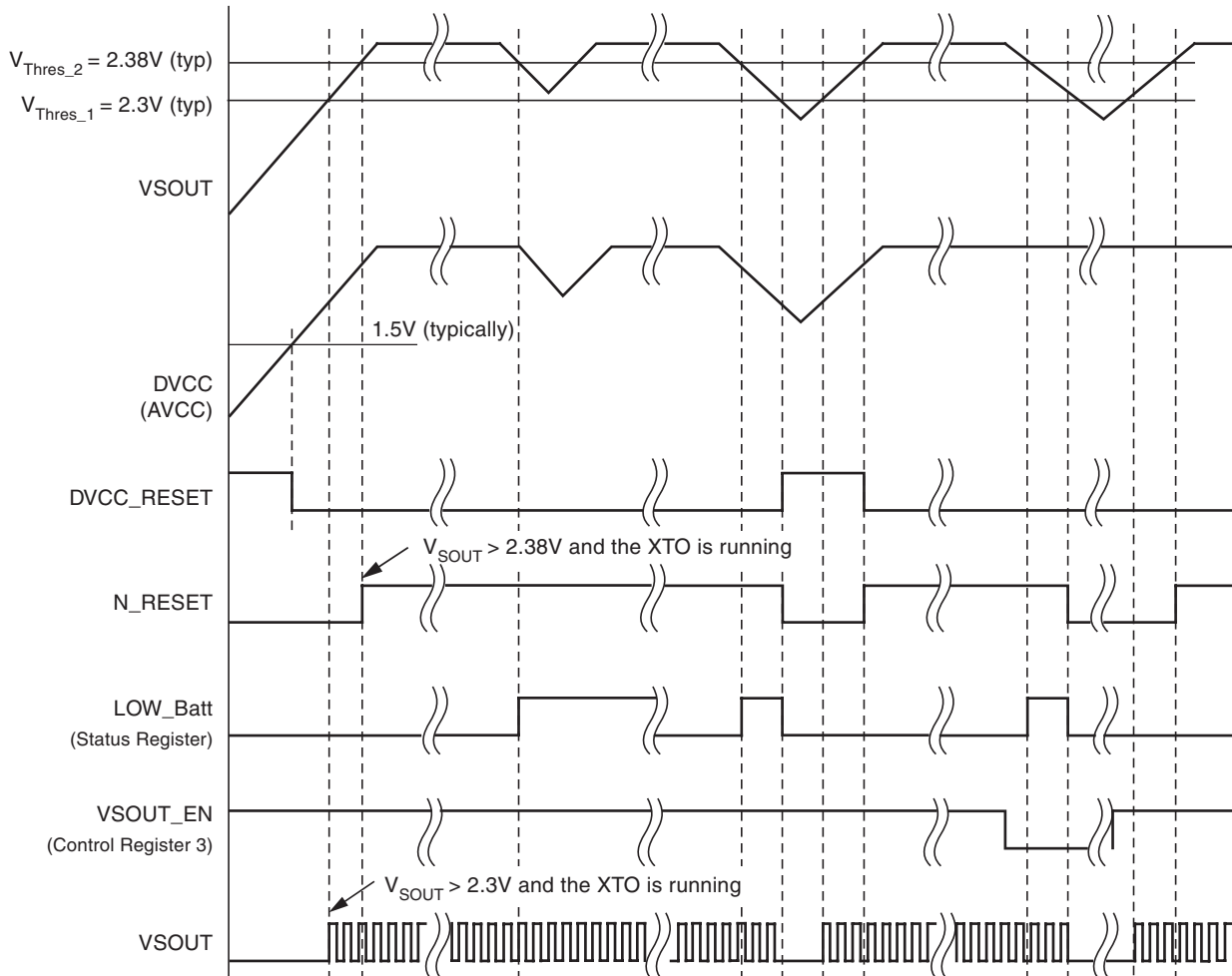
Figure 5-3. Reset Timing
