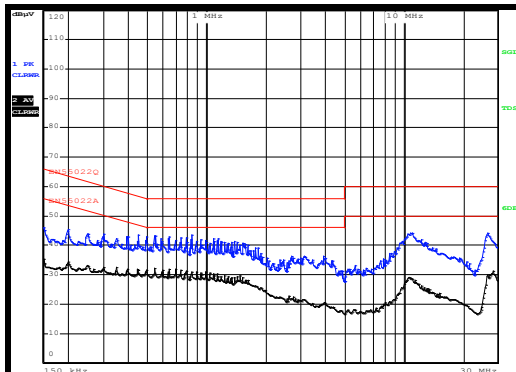
Conducted EMI
