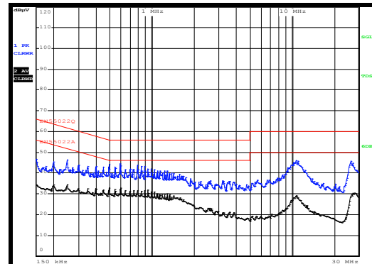
Conducted EMI
