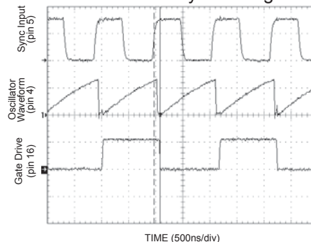
Figure 6. Sync Waveform
