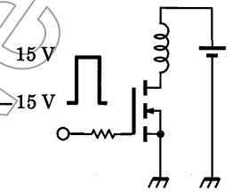
TEST CIRCUIT
