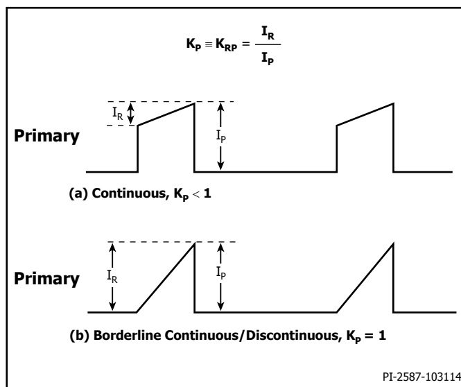
Figure 20. Continuous Mode Current Waveform, K_p \leq 1 .
