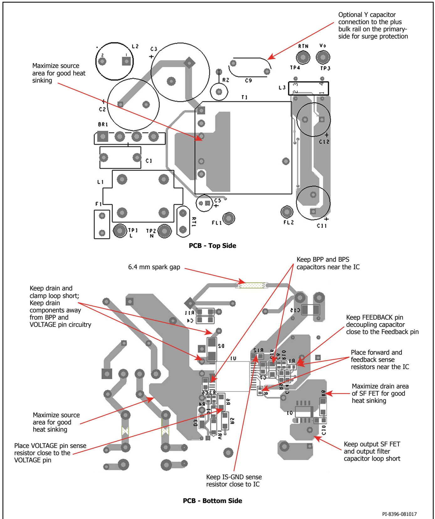
Figure 19. PCB.
