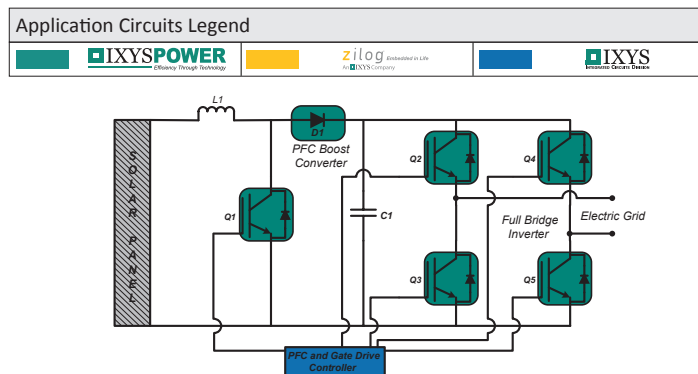
Figure 1: Solar Inverter
