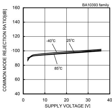
Fig.39 Common Mode Rejection Ratio - Supply Voltage
