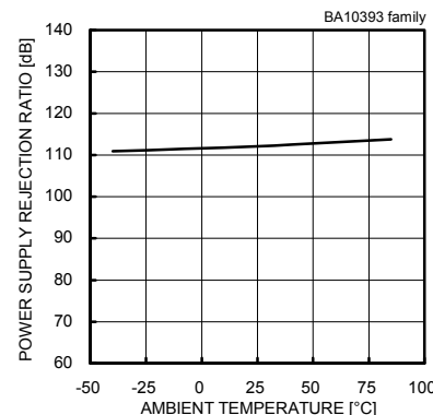
Fig.41 Power Supply Rejection Ratio - Ambient Temperature
