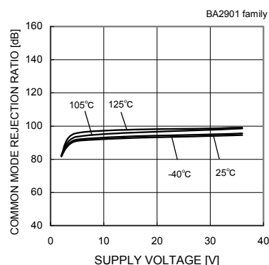
Fig.102 Common Mode Rejection Ratio - Supply Voltage
