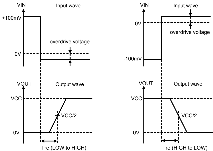
Fig.113 Response Time
