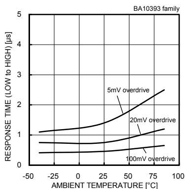
Fig.42 Response Time (Low to High) - Ambient Temperature (VCC=5[V],VRL=5[V],RL=5.1[kΩ])
