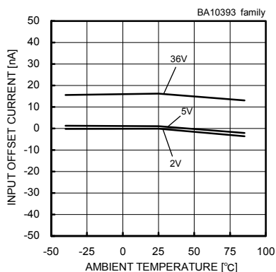
Fig.36 Input Offset Current - Ambient Temperature
