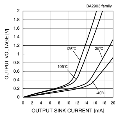
Fig.69 Low Level Output Voltage - Output Sink Current (VCC=5[V])
