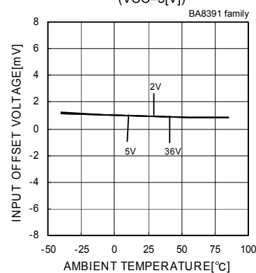
Fig.9 Input Offset Voltage - Ambient Temperature
