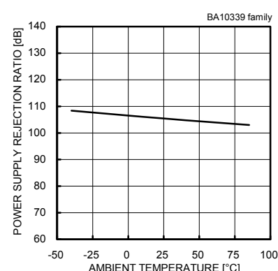
Fig.61 Power Supply Rejection Ratio - Ambient Temperature
