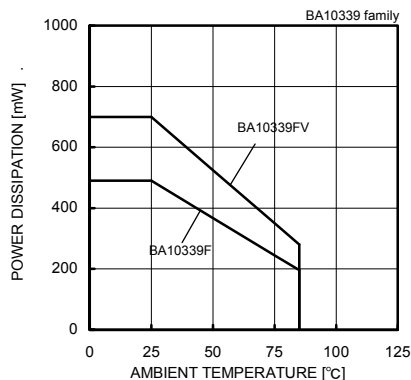
Fig.44 Derating Curve
