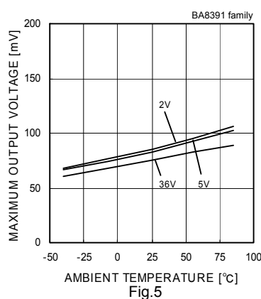
Fig.5 Output Saturation Voltage - Ambient Temperature (IOL=4[mA])
