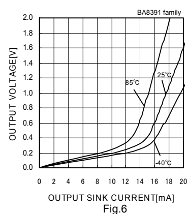
Fig.6 Low Level Output Voltage - Output Sink Current (VCC=5[V])
