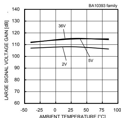
Fig.38 Large Signal Voltage Gain - Ambient Temperature
