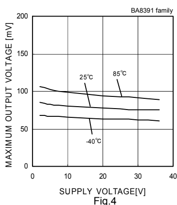
Fig.4 Output Saturation Voltage - Supply Voltage (IOL=4[mA])
