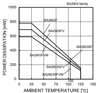
Fig.64 Derating Curve
