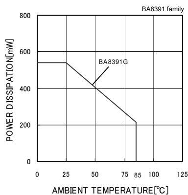
Fig.1 Derating Curve
