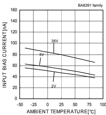
Fig.11 Input Bias Current - Ambient Temperature
