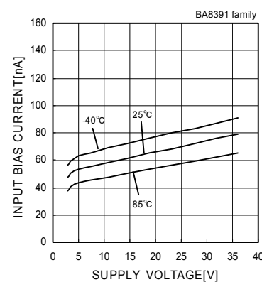
Fig.10 Input Bias Current - Supply Voltage
