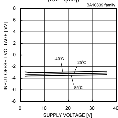
Fig.51 Input Offset Voltage - Supply Voltage
