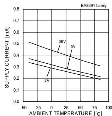
Fig.3 Supply Current - Ambient Temperature
