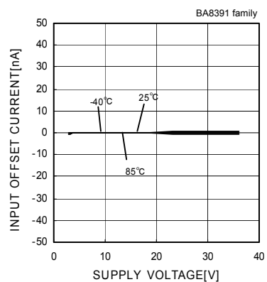
Fig.12 Input Offset Current - Supply Voltage
