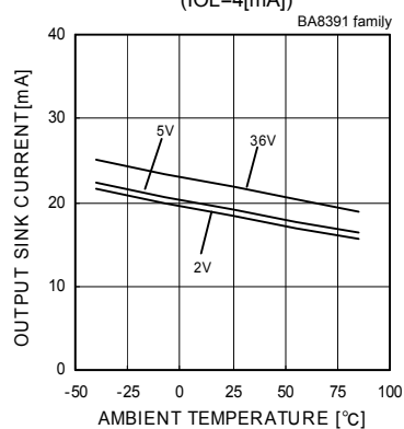
Fig.7 Output Sink Current - Ambient Temperature (VOUT=1.5[V])
