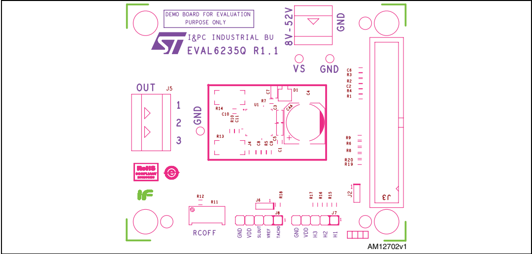
Figure 3. EVAL6235Q - layout (silk screen)
