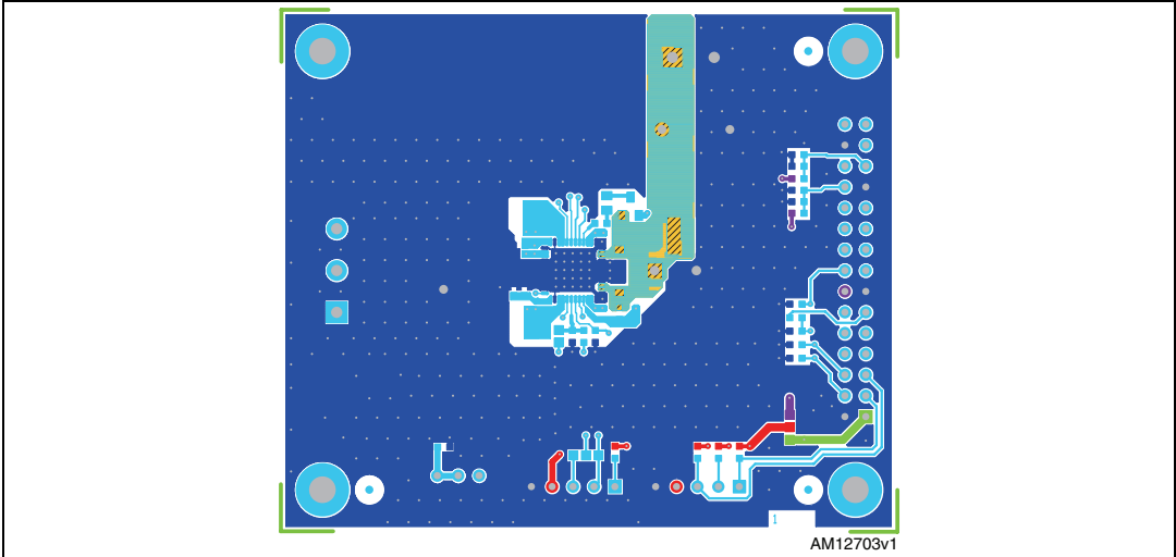
Figure 4. EVAL6235Q - layout (top layer)
