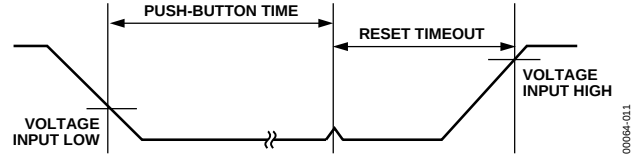
Figure 12. Push-Button Reset Timing Diagram
