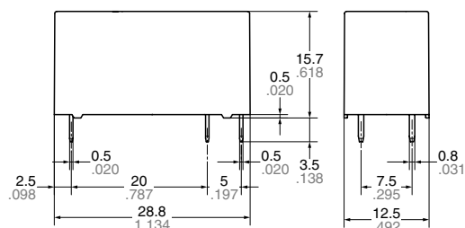
External dimensions
