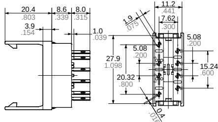
External dimensions
