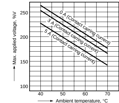
6.-(1) Ambient temperature vs Max. applied voltage Tested sample: NC2D-P-DC24 V (2 Form C slim single side stable)
