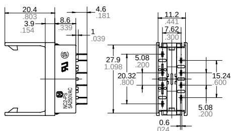
External dimensions
