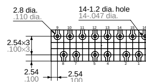
PC board pattern
