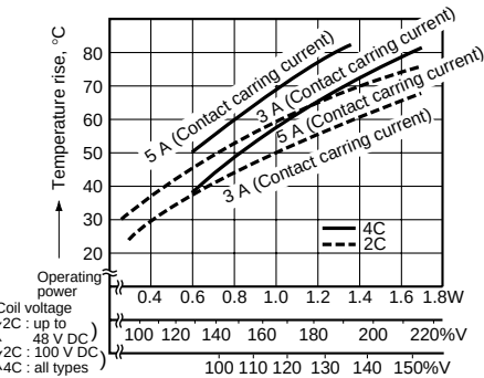
2. Temperature rise characteristics (single side stable) Measured portion: Inside the coil
