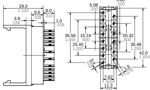
External dimensions
