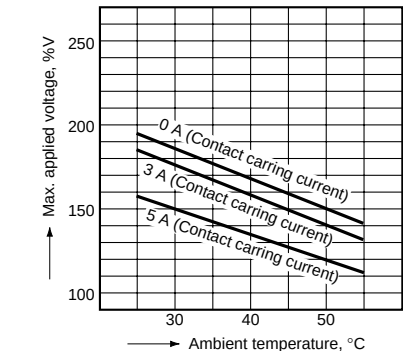
6.-(2) Ambient temperature vs Max. applied voltage Tested sample: NC2D-P-DC110 V (2 Form C slim single side stable), NC4D-P-DC24 V (4 Form C slim single side stable)
