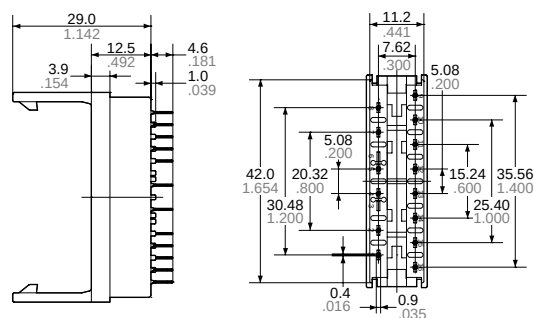
External dimensions
