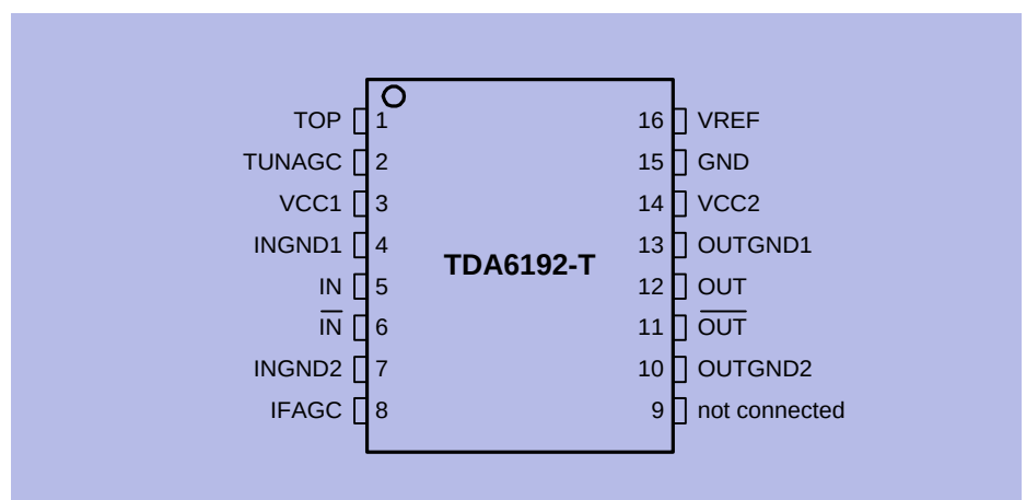
Figure 3-2 TDA6192-T, Pin Configuration
