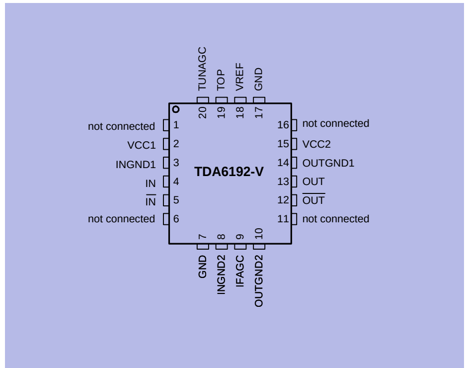
Figure 3-1 TDA6192-V, Pin Configuration
