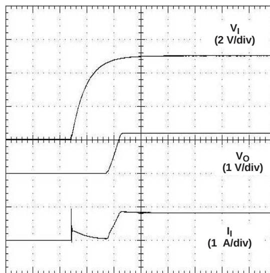
Figure 20. Power-Up Waveform
