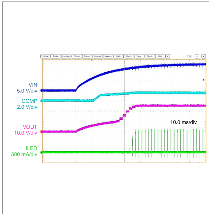
Figure 31. VIN Power ON (PWM Mode)
