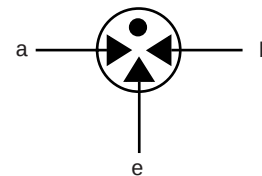
3 ELECTRODE GDT
