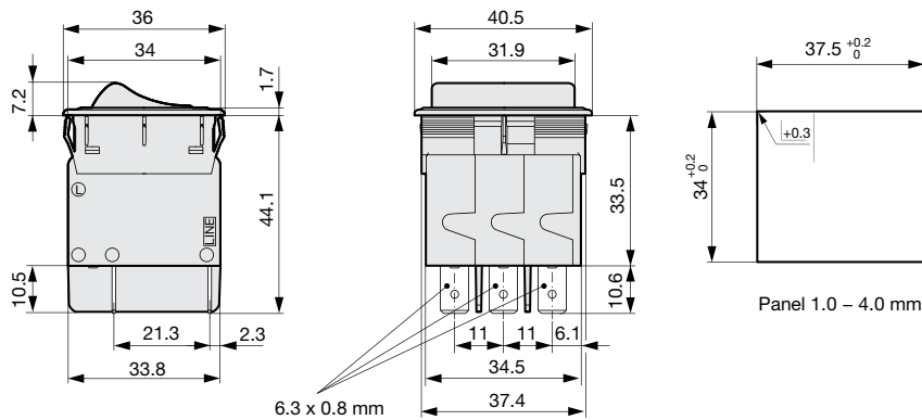
3-pole, 3 bimetal, non illuminated
