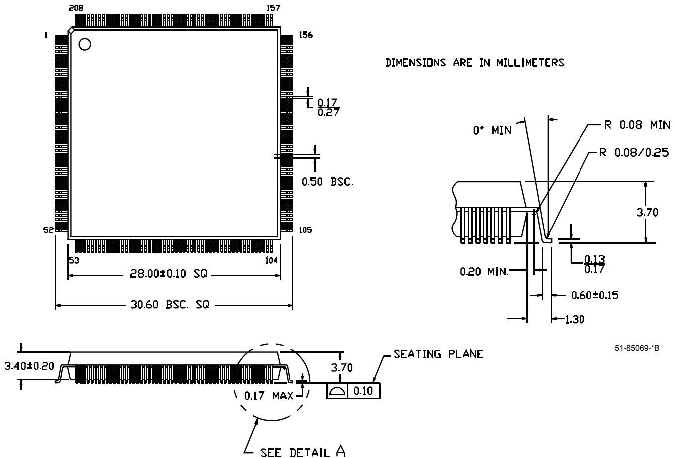
208-Lead Enhanced Quad Flat Pack (EQFP) NT208 208-Lead Lead-Free Enhanced Quad Flat Pack (EQFP) NT208
