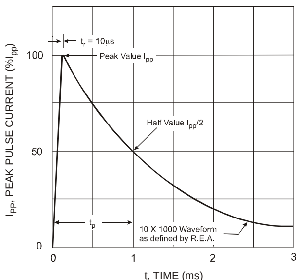
Fig. 4 Pulse Waveform
