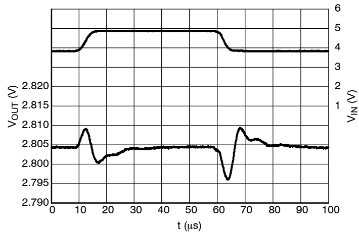
Figure 27. Line Transients, 2.8 V Version, t_R = t_F = 5 \mu s, I_{OUT} = 30 mA
