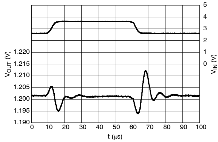
Figure 26. Line Transients, 1.2 V Version, t_R = t_F = 5 \mu s, I_{OUT} = 30 mA
