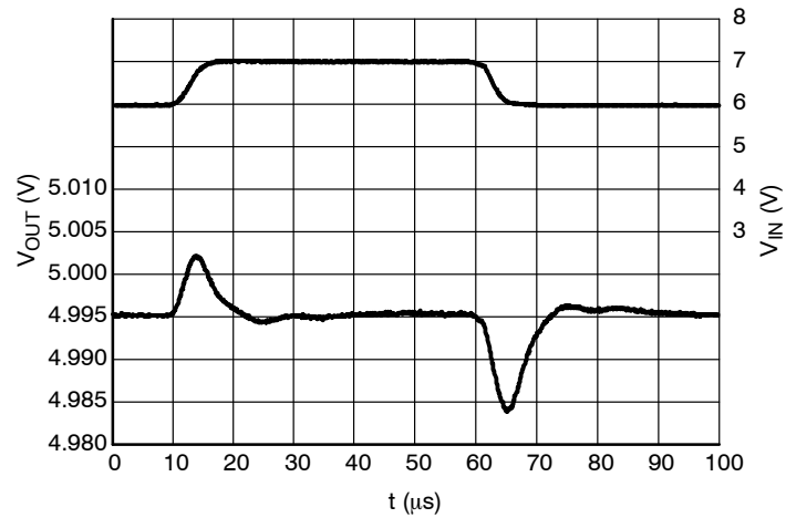
Figure 28. Line Transients, 5.0 V Version, t_R = t_F = 5 \mu s, I_{OUT} = 30 mA
