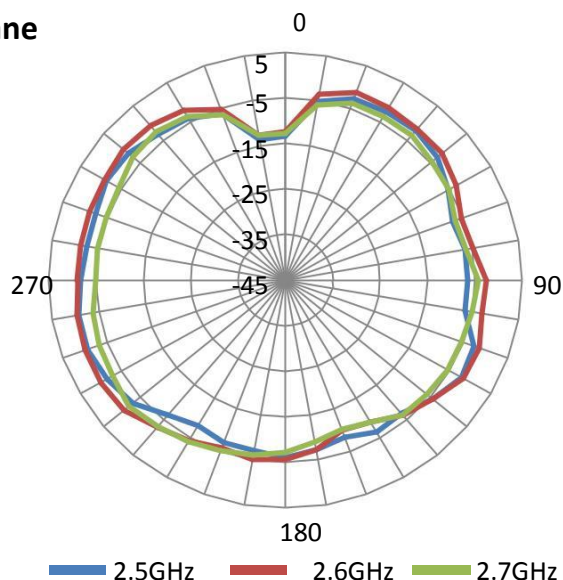
E Plane - 2500 - 2700MHz
