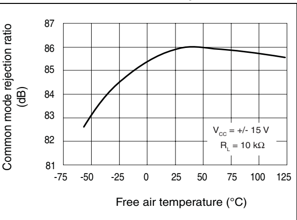
Figure 11. Common-mode rejection ratio versus free air temperature
