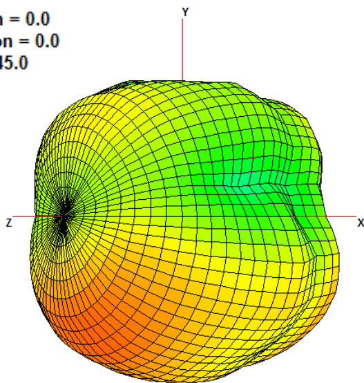
Figure 13. 3D Radiation Pattern at 1805 and 1910 MHz of the Warrior PA.711.A Antenna on MIMO PAD.71X.A
