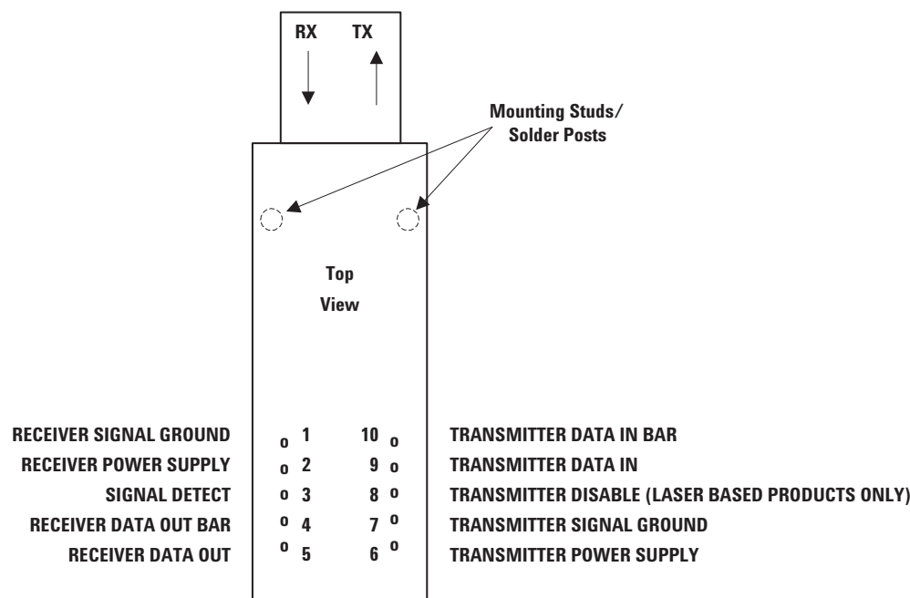
Figure 3. Pin Out Diagram.
