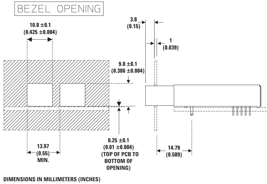
Figure 10. Recommended Panel Mounting
