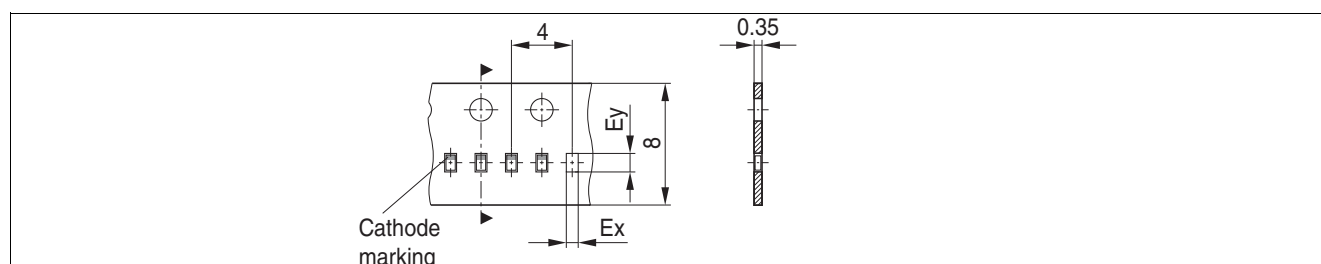
Figure 6-3 PG-TSSLP-2-1: Packing
