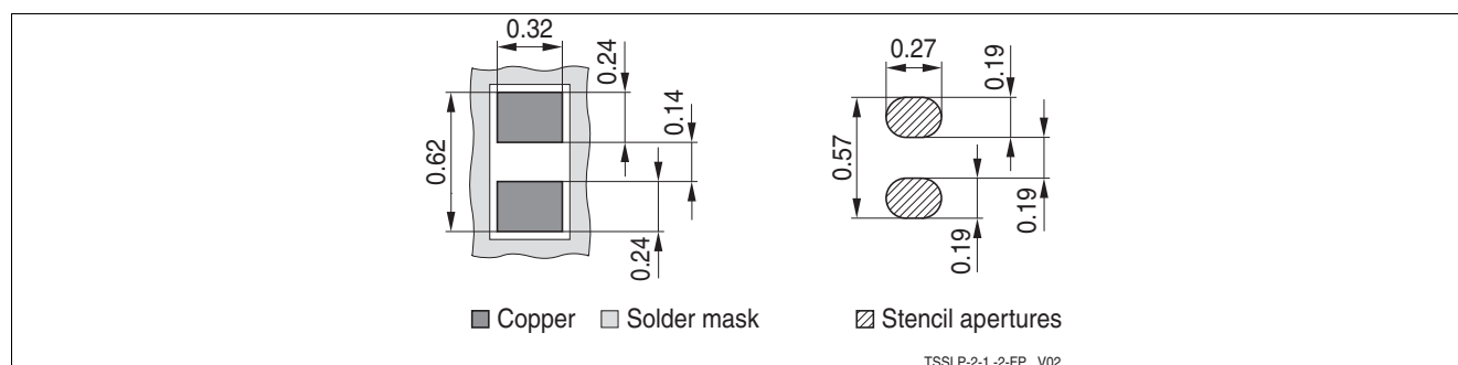
Figure 6-2 PG-TSSLP-2-1: Footprint
