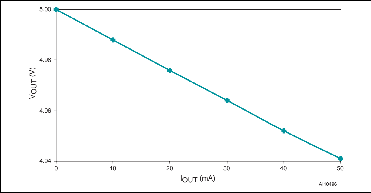
Figure 27. Output Voltage vs. Load Current ( V_{CC} = 5V ; V_{BAT} = 2.8V ; T_A = 25^\circ C )
