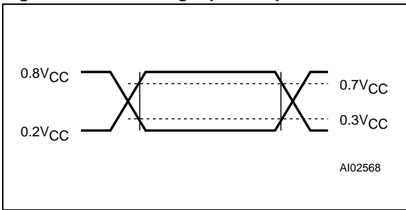
Figure 36. AC Testing Input/Output Waveforms
