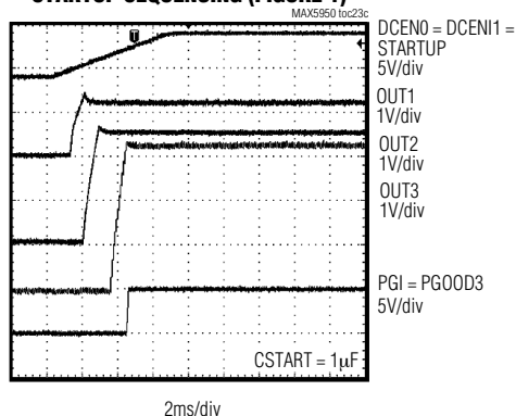
STARTUP SEQUENCING (FIGURE 1)
