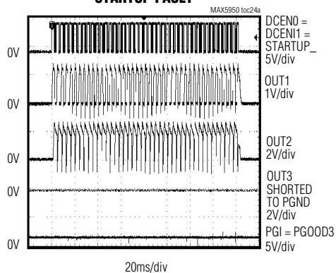
STARTUP FAULT
