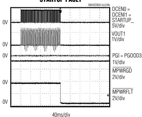
STARTUP FAULT
