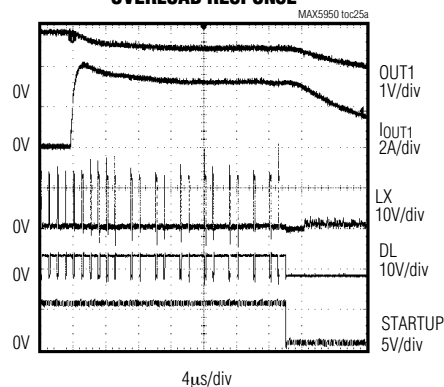
OVERLOAD RESPONSE
