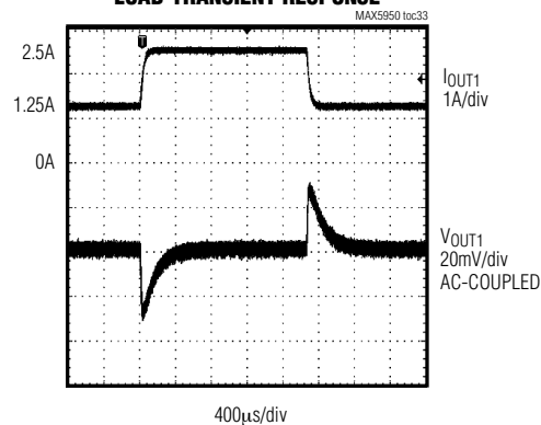
LOAD-TRANSIENT RESPONSE
