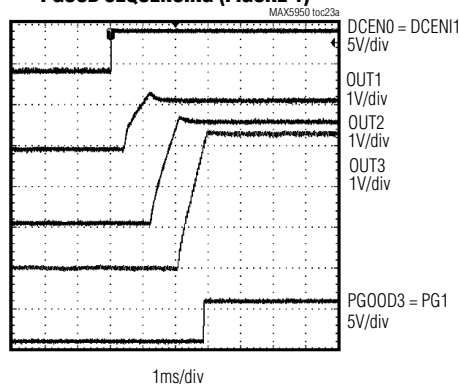
PGOOD SEQUENCING (FIGURE 1)
