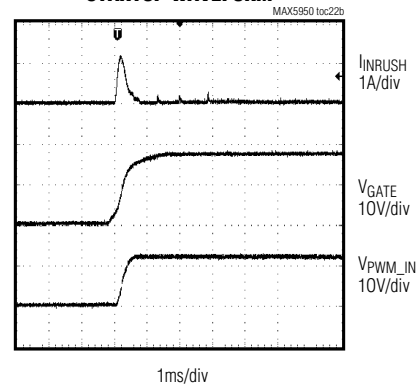
STARTUP WAVEFORM
