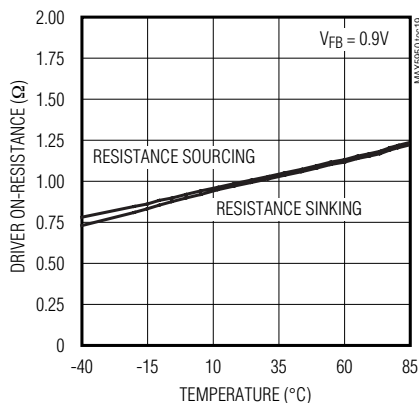
DL, DH DRIVER ON-RESISTANCE vs. TEMPERATURE
