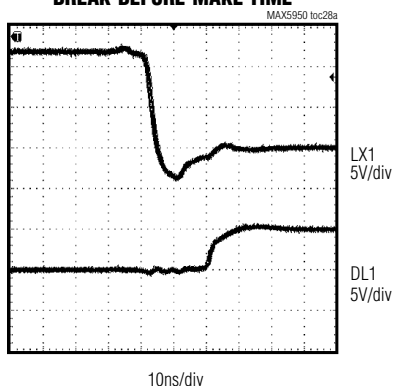
BREAK-BEFORE-MAKE TIME
