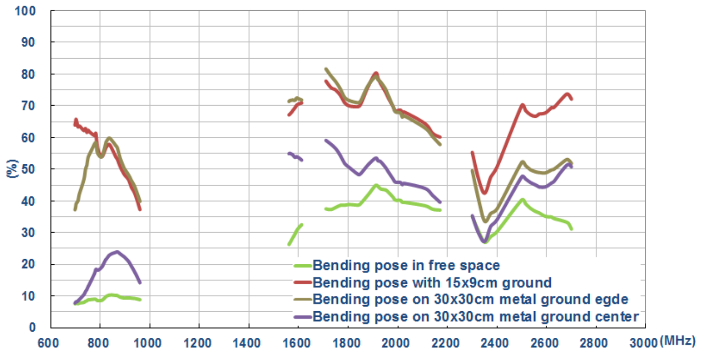
Figure5. Efficiency of TG.08 antenna with bent Position
