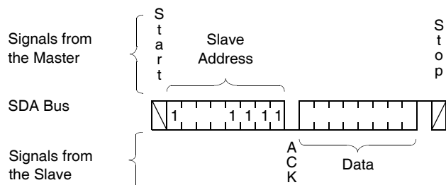
Figure 15. Current Address Read Sequence
