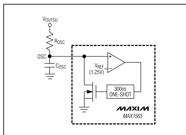
Figure 4. Master Oscillator
