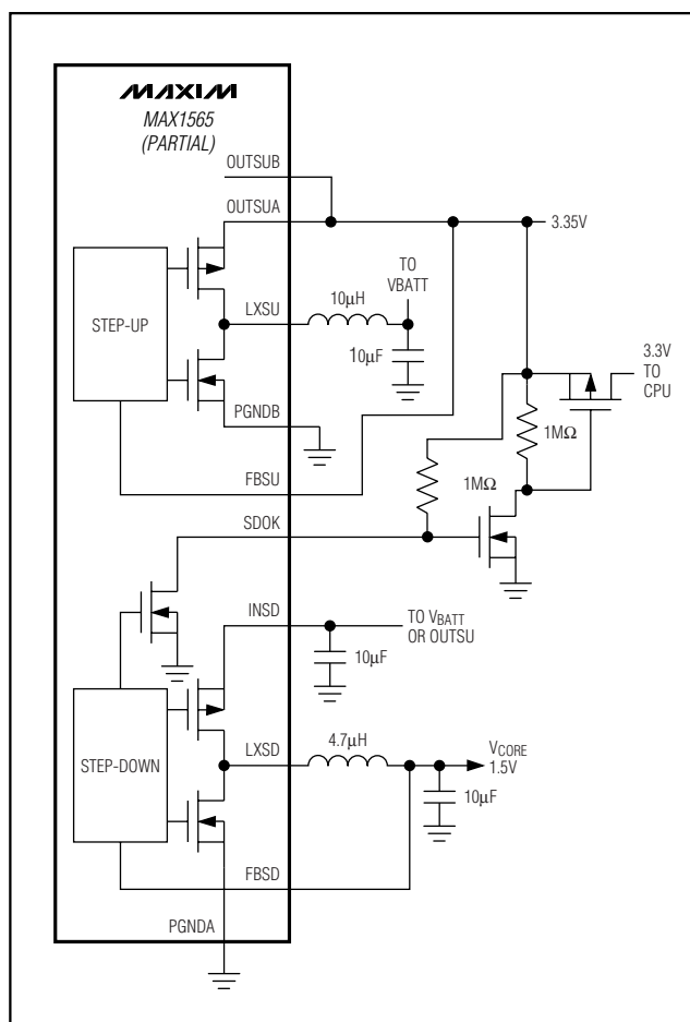
Figure 12. Using SDOK to Gate 3.3V Power to CPU After the Core Voltage is OK
