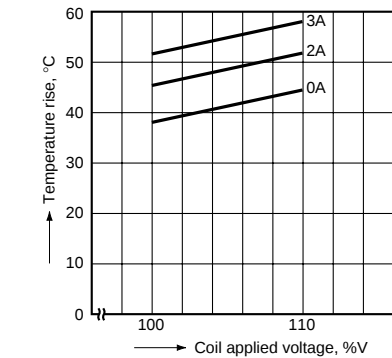
6-(1). Influence of adjacent mounting (1 Form C)
