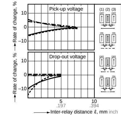
6-(1). Influence of adjacent mounting (1 Form C)
