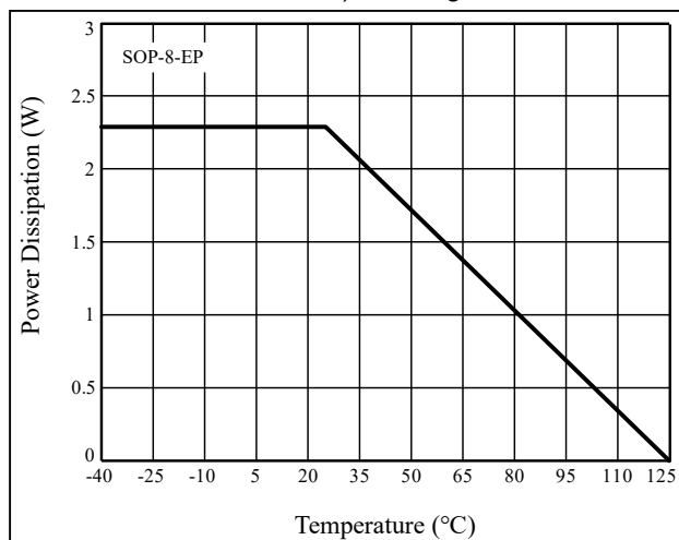
Figure 34 Dissipation Curve
