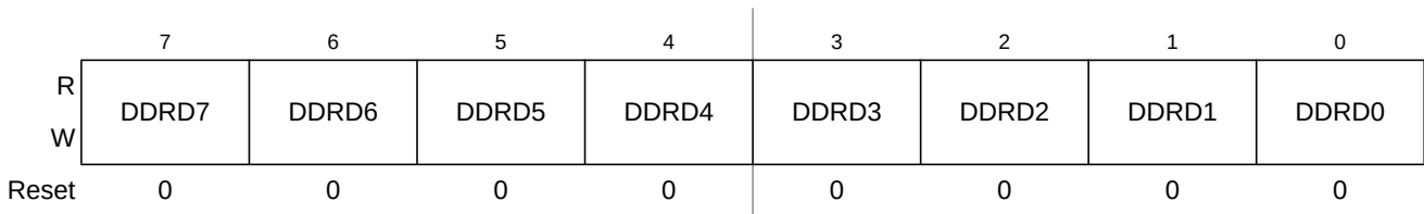
Figure 22-10. Port D Data Direction Register (DDRD)
