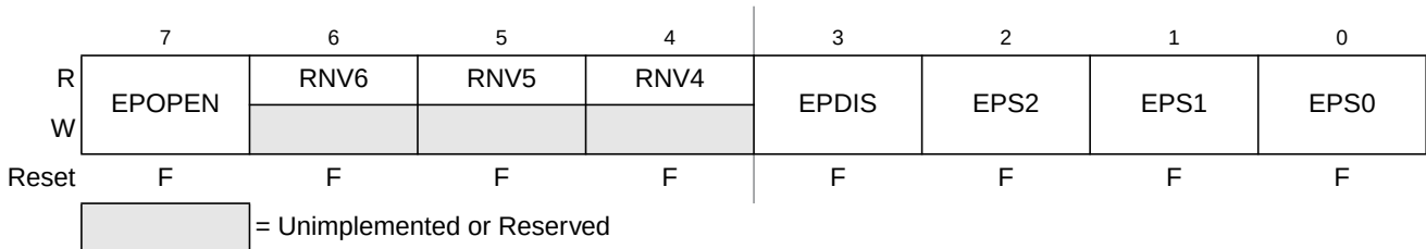
Figure 25-8. EEPROM Protection Register (EPROT)
