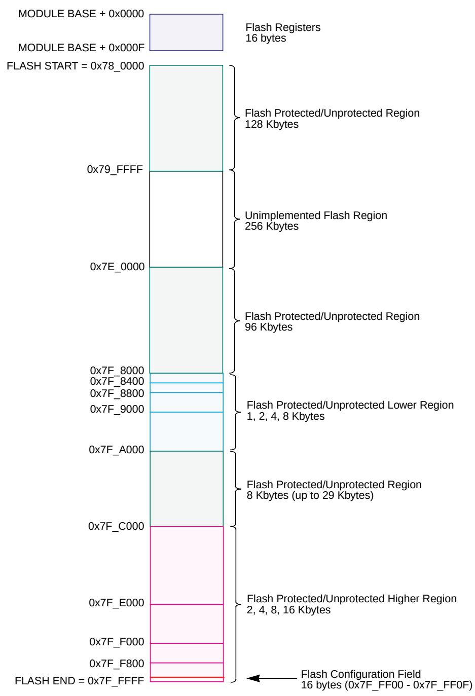
Figure 28-2. Flash Memory Map
