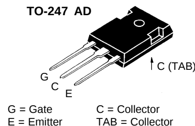
TO-247 AD
