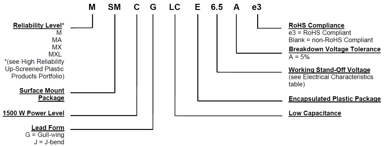
Figure 2-1. Part Nomenclature
