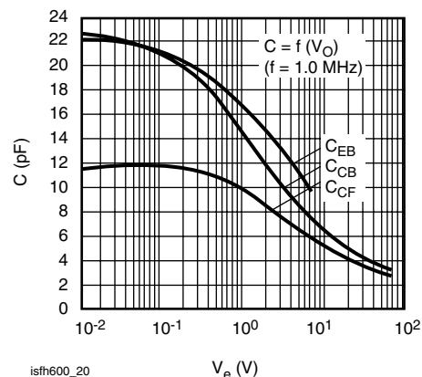
Fig. 20 - Transistor Capacitance
